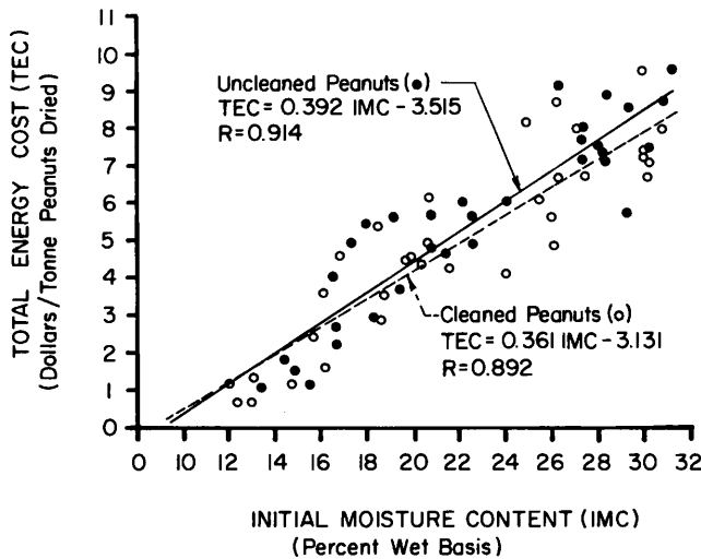
Fig. 8. Comparison to total energy costs for drying U and C peanuts.
