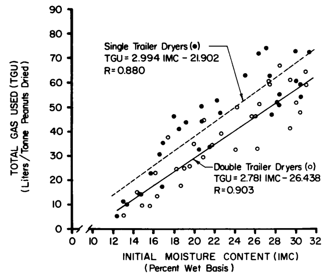
Fig. 3. Comparison of the effects of initial m.c. on total gas used during drying with ST and DT dryers.
