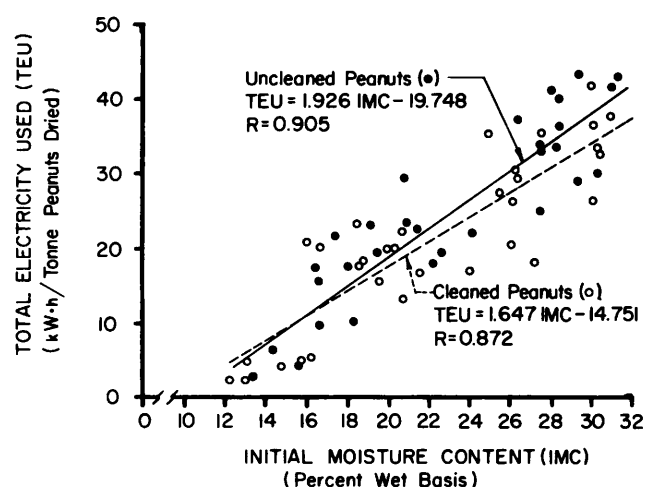
Fig. 5. Comparison of the effects of initial m.c. on total electricity used for drying Uc and C peanuts.
