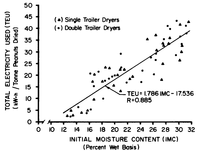
Fig. 2. The effect of initial m.c. on total electricity used for drying peanuts with ST and DT dryers.
