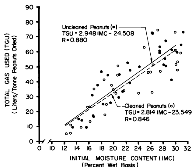
Fig. 6. Comparison of the effects of initial m.c. on total gas used for drying Uc and C peanuts.
