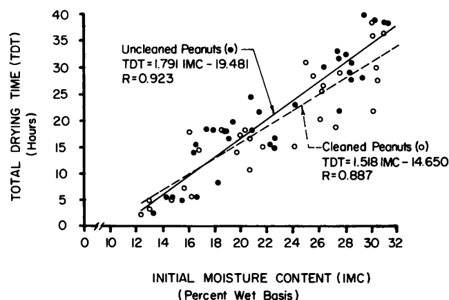
Fig. 7. Comparison of the effects of initial m.c. on total drying times for drying Uc and C peanuts.
