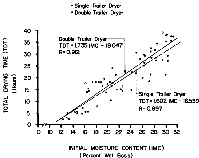
Fig. 1. The effect of initial m.c. on total drying times of peanuts dried with ST and DT dryers.
