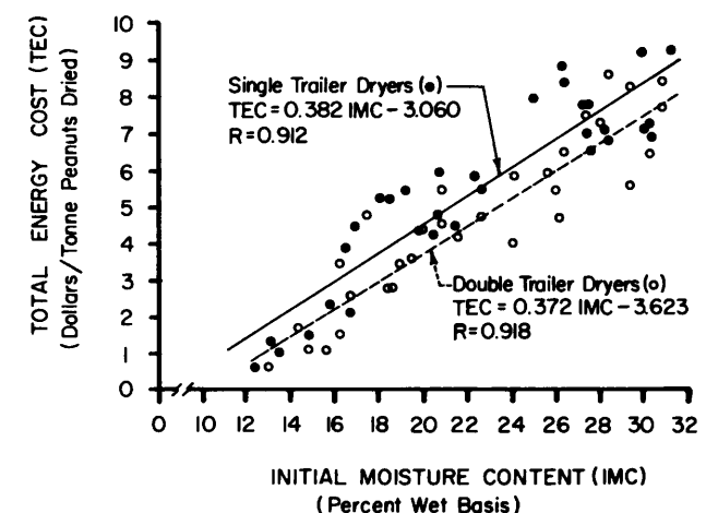
Fig. 4. Comparison of the effects of initial m.c. on total energy costs for drying with ST and DT dryers.
